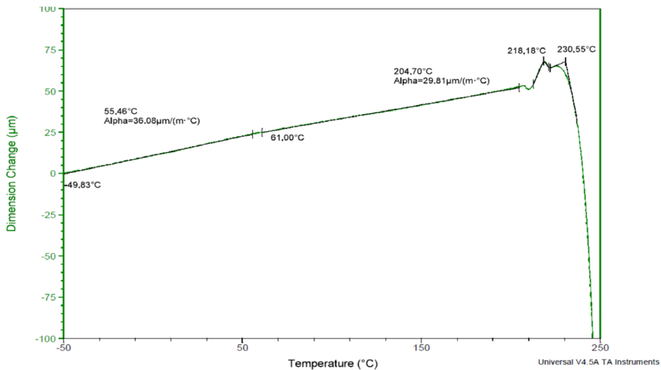
Figure 3: Dimension change data as a function of temperature for the ULTEM™ 1010 resin On Edge (XZ) sample.
