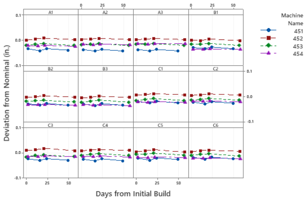
Figure 10 - Large (>8 inch) Features for ASA 9-inch check part on Fortus 450mc.
