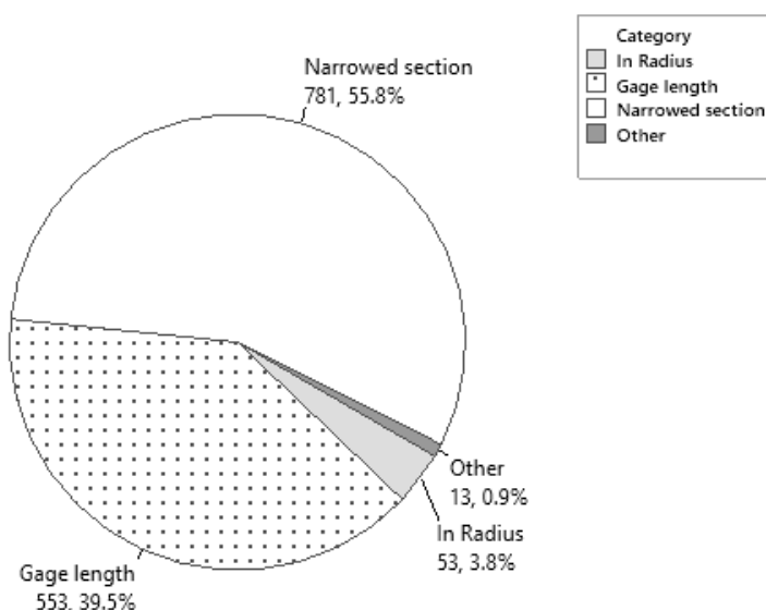
Figure 15 - Summary of coupon break locations including all materials and machines.
