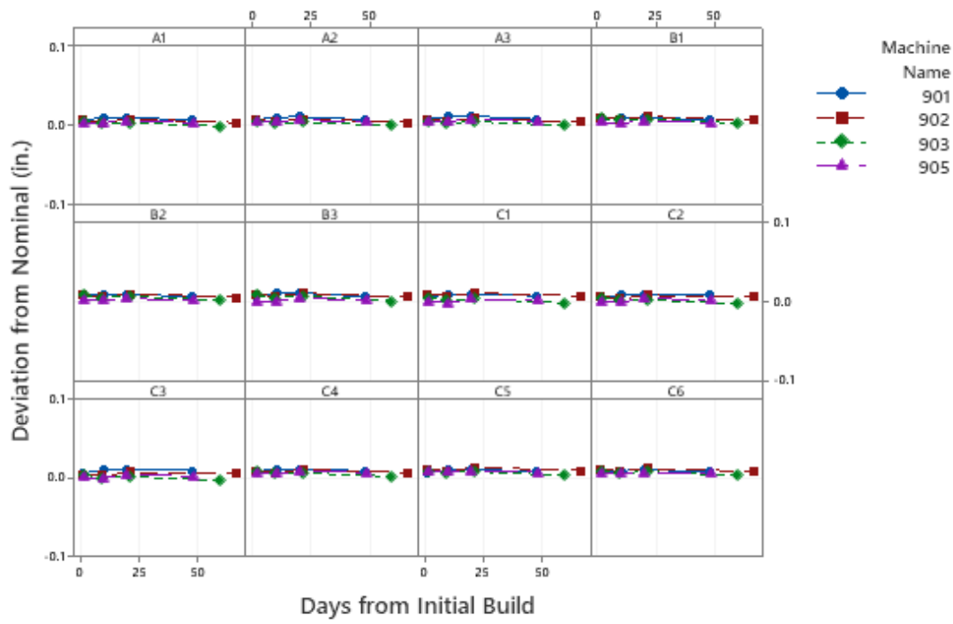
Figure 11 - Large (>8 inch) Features for ASA 9-inch check part on F900.
