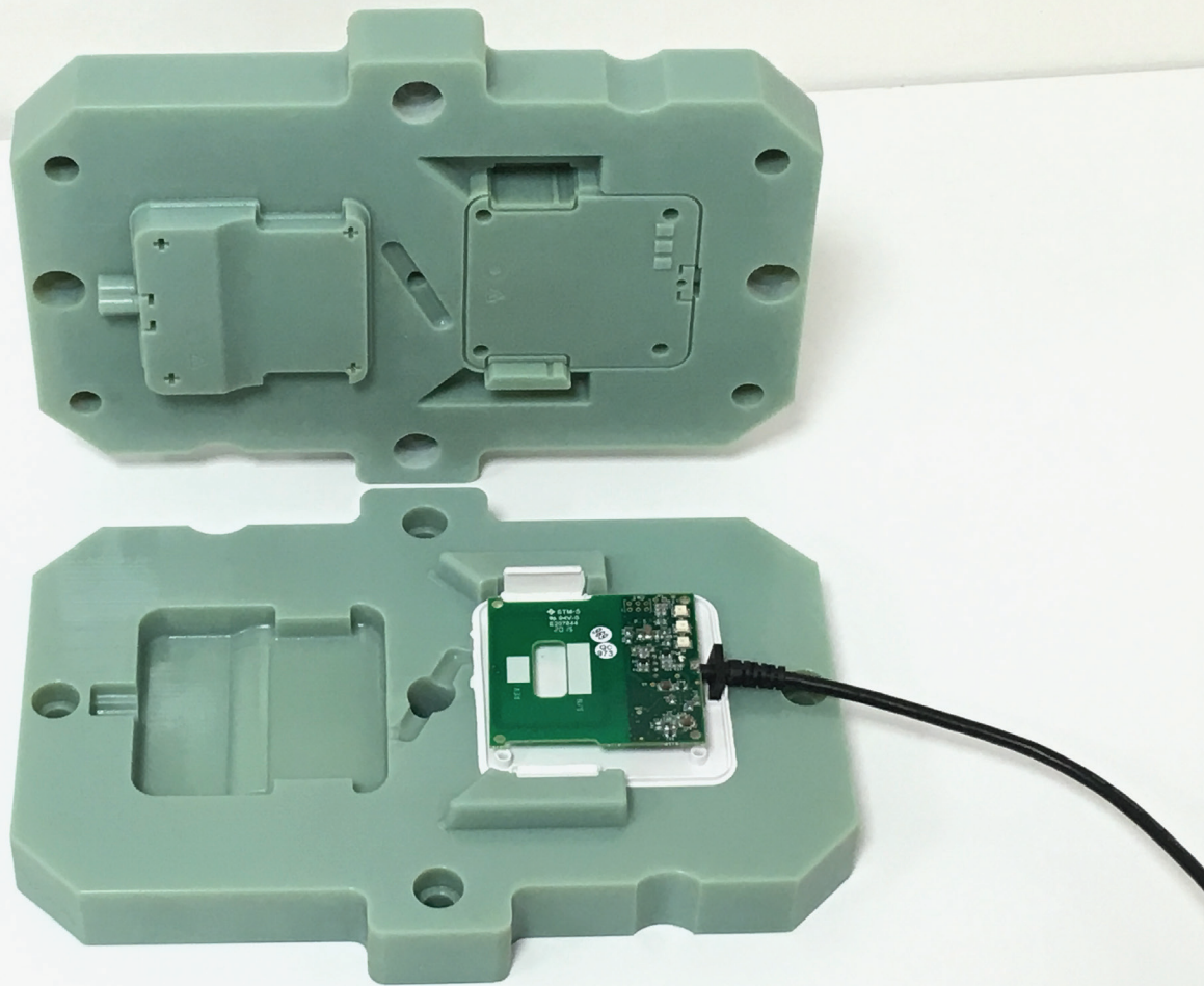
3D printed injection molds created in Digital ABS material.
