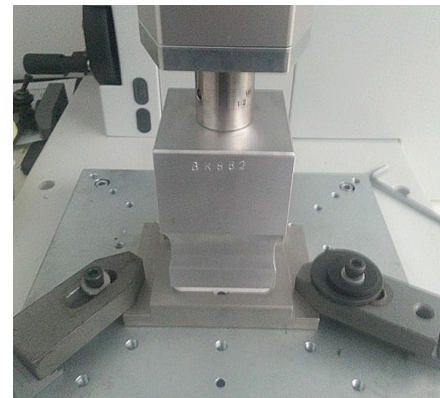
Welding process for injected parts
