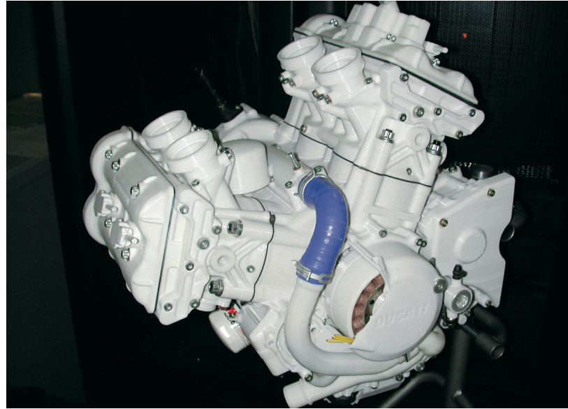
The Desmosedici's engine was prototyped almost entirely from polycarbonate using the FDM process.
