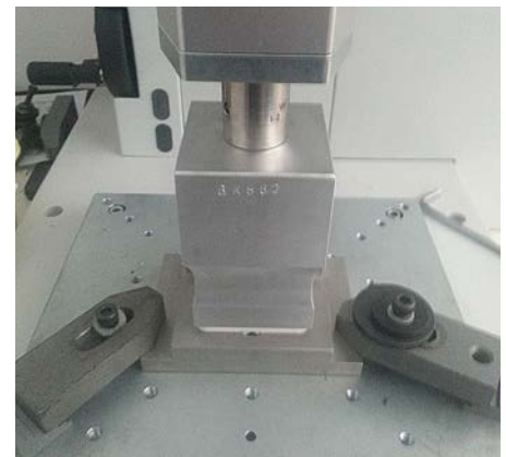
Welding process for injected parts
