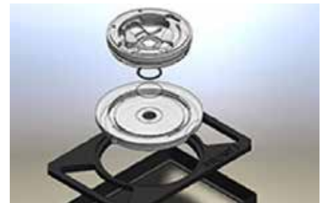
A 3D rendering of perfusion chamber's different parts
