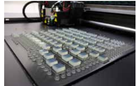
The perfusion tray was 3D printed in bio-compatible material since it will come into direct contact with cells and tissues.
