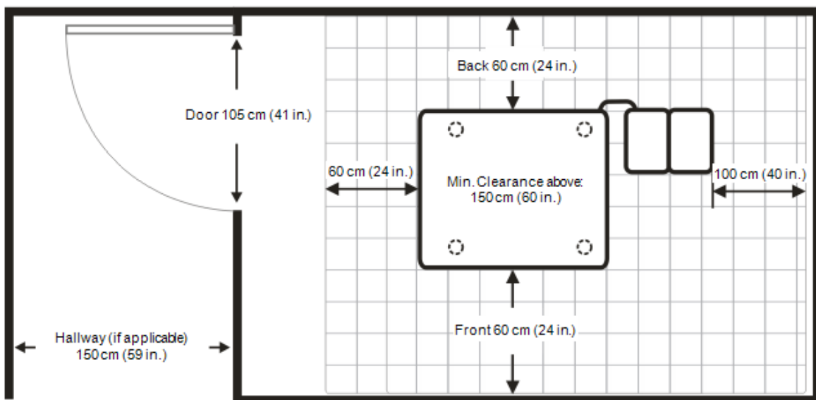
Figure 3 Printer floor plan (sample, not to scale)
